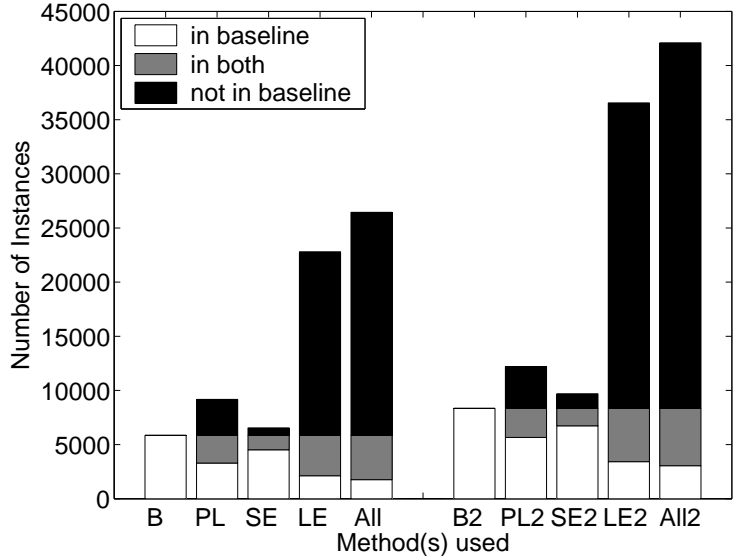
Experiment 9: The number of correct instances of City at precision .90 and at precision .80 for baseline KNOWITALL and extensions to the baseline system. Each extension increased recall, with List Extractor giving more than a 4-fold improvement.
