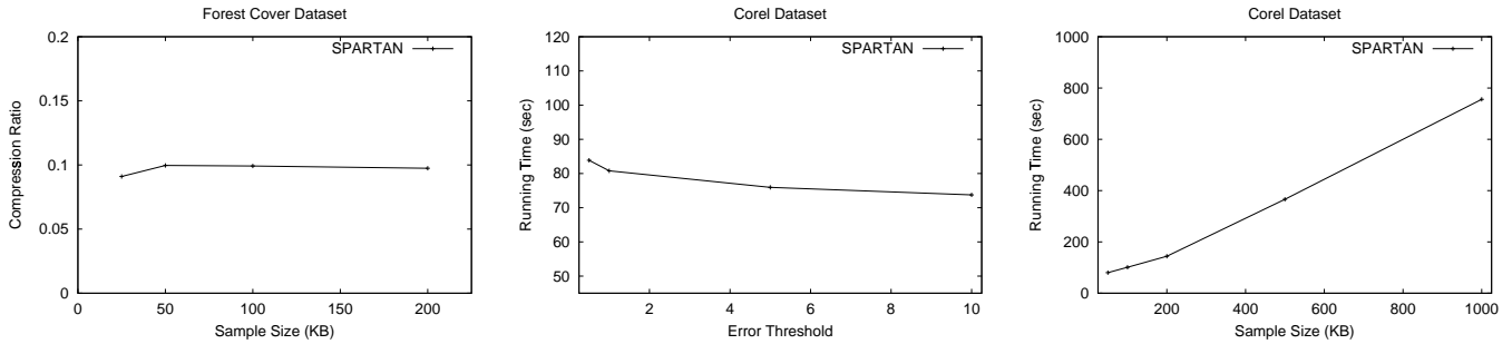
Figure 6: Effect of Error Threshold and Sample Size on Compression Ratio/Running Time.
