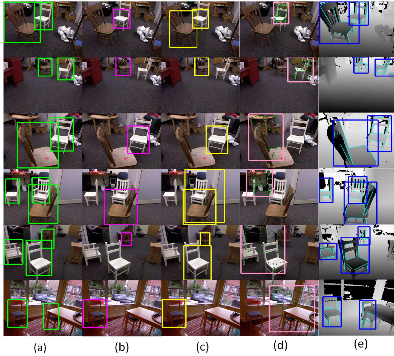
Fig. 6. Some chair detection results. (a) ground truth, (b) DPM [22], (c) DPM-SIZE [21]. (d) PAS [3] with transformed model shown with dots, and (e) The proposed method with results shown on depth map to stress that they are obtained in 3D.
