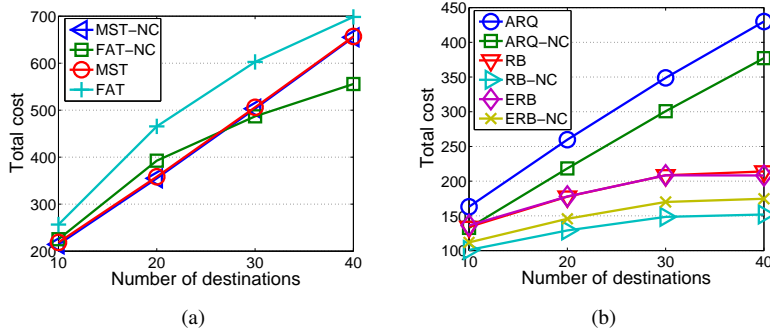
FIGURE 12 (a) Multi-hop broadcasting; n = 20 . (b) One-hop broadcasting with lossy feedbacks; P \in [0.4, 0.7] ; n = 20 .
