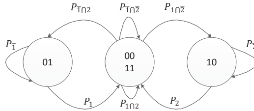
FIGURE 4 Markov chain for two destination nodes.
