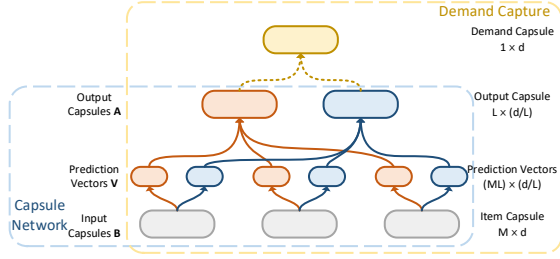
Figure 3: The process of the capsule network.
