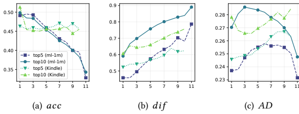
Figure 10: Comparison on different user group.
