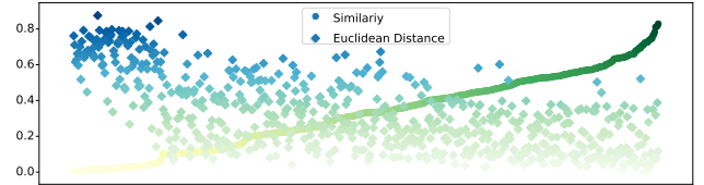
(b) Kindle
