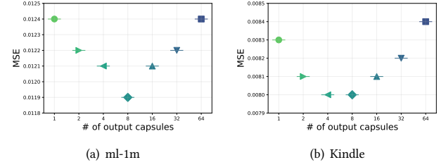
Figure 8: Effects of the number of output capsules.
