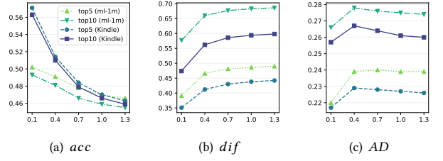
Figure 9: Effects of m_{base}
