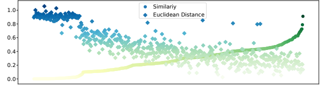
(a) ml-1m
