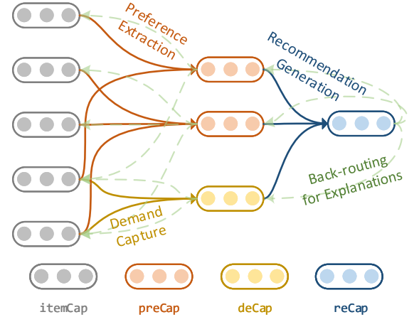
Figure 2: The framework of DESR.
