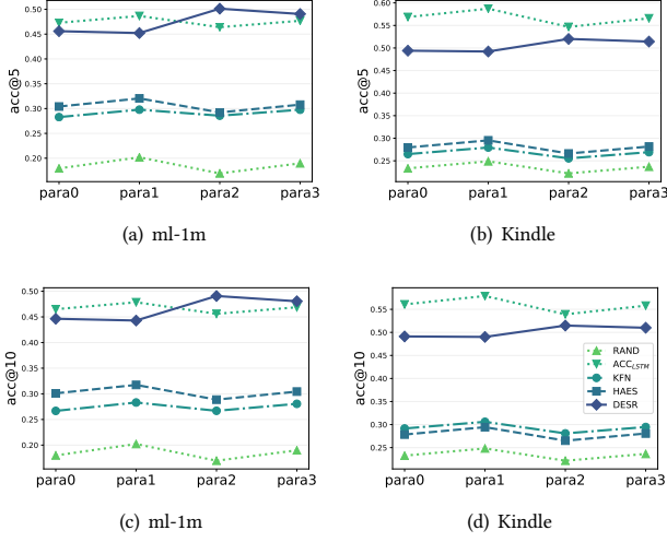
Figure 6: Effects of parameters on acc. (para0: \eta = 0.5, \theta = 0.5 ; para1: \eta = 0.5, \theta = 1 ; para2: \eta = 1, \theta = 0.5 ; para3: \eta = 1, \theta = 1 .)
