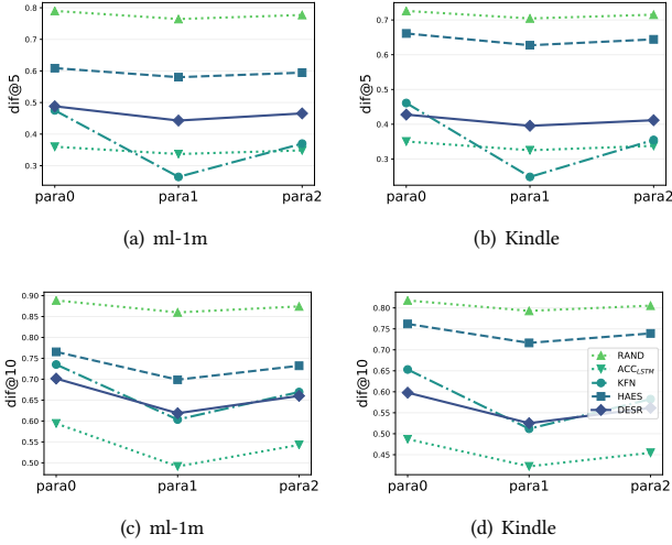
Figure 7: Effects of parameters on dif. (para0: \lambda = 0.5, \gamma = 1 ; para1: \lambda = 1, \gamma = 0.5 ; para2: \lambda = 1, \gamma = 1 .)
