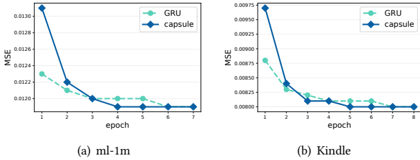
Figure 11: Comparison between the capsule network and GRU on capturing users' short-term demands.
