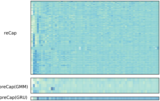
Figure 12: Comparison between GMM and GRU on capturing users' long-term preferences.
