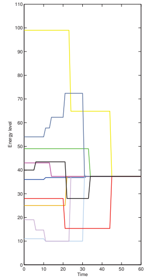
Fig. 7: Energy level of each EV over time using LAY (10 EVs are represented by 10 different colors)
