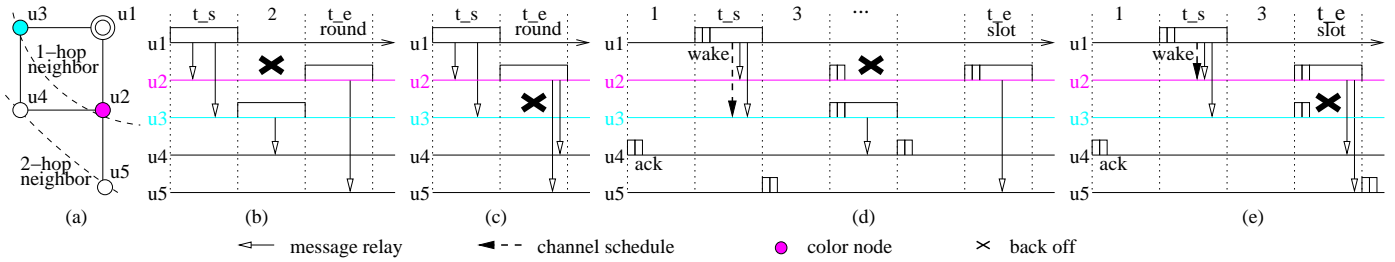
Fig. 2. (a) Broadcasting (from u_1 ) with a conflict at u_4 . (b) Deferred broadcasting and (c) the minimum latency broadcasting under the network model of the round-based system. (d) Deferred broadcasting and (e) the optimal solution under the duty cycle model.
