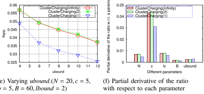
Fig. 6: Impact of various parameters in Random-Setting
