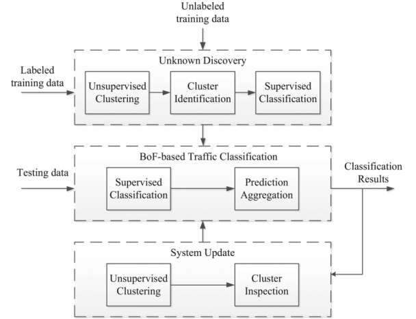
Fig. 1. RTC framework.
