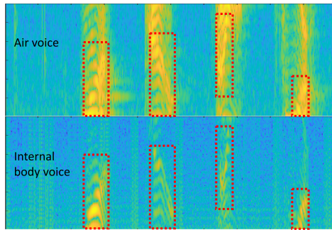
Fig. 4. The spectrograms of voices through air and internal body.
