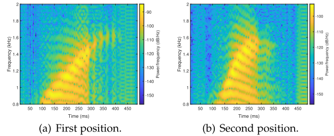
Fig. 21. Spectrograms of body voice when the sensor is at two positions.
