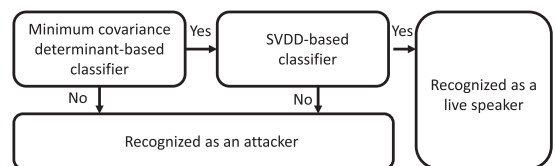
Fig. 12. Workflow of classification model.
