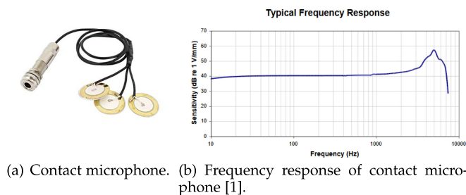
Fig. 3. Contact microphone and its frequency response.
