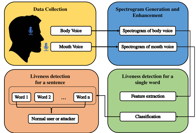
Fig. 5. System pipeline.
