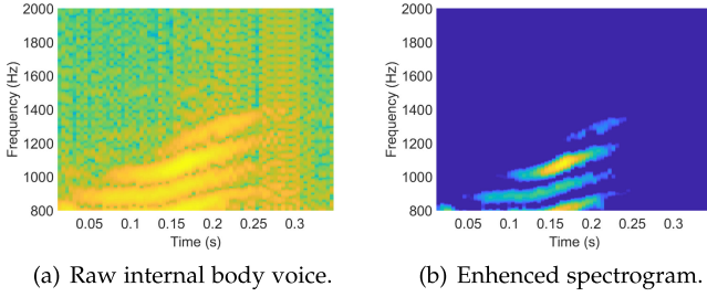
Fig. 6. Spectrogram enhancement.
