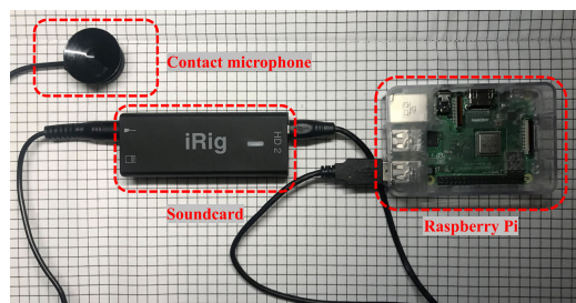
Fig. 13. Testbed for collecting internal body voice.
