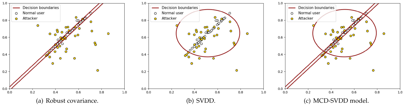
Fig. 11. Decision boundaries of different classifiers.
