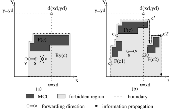
Figure 4: (a) A “must-take” detour. (b) A sample of complete information broadcasting and a correct routing decision based on such information.
