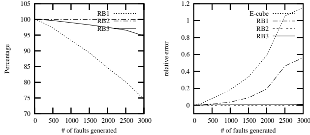
Figure 9: (a) Percentage of success in finding the shortest-path. (b) Relative error of routing path achieved to the shortest-path.
