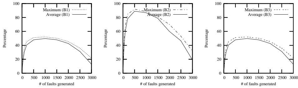
Figure 8: Percentage of nodes involved in information propagation to the total safe nodes in the meshes.
