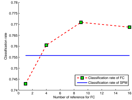
Figure 6. The classification rate of FC for different numbers of reference points. The blue curve is the classification rate of SPM encoded with RBC coding. It is shown as a baseline.
